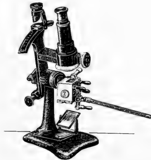
REFRACTOMETER USED FOR DETERMINING REFRACTIVE INDEX OF FREE OIL IN CANNED SALMON.
